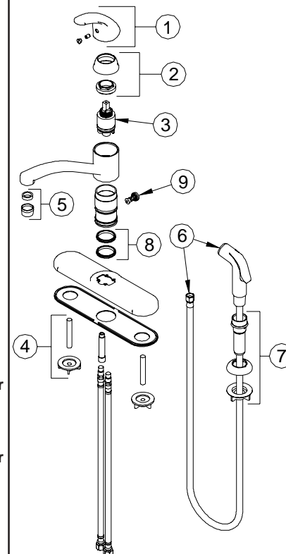
Spray hose & handset Assy. (Model Z7872C only)
