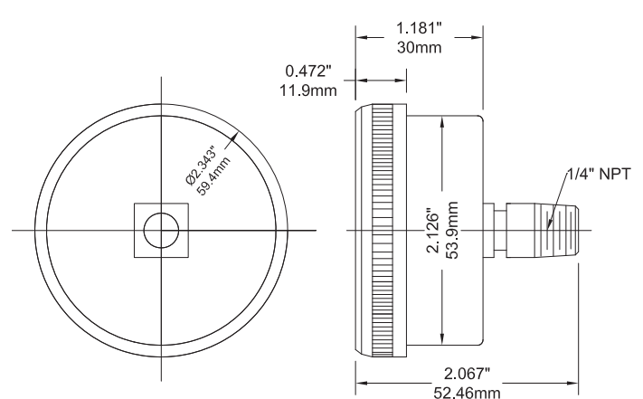
2" Back Connection
