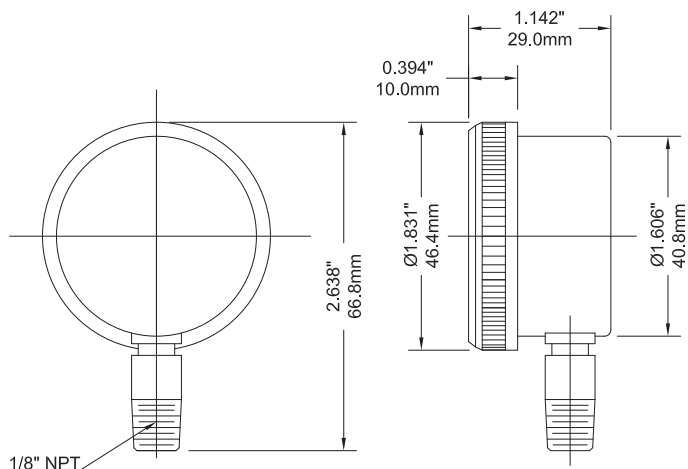
1.5" Bottom Connection
