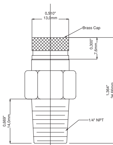
0.25" Test Plug
