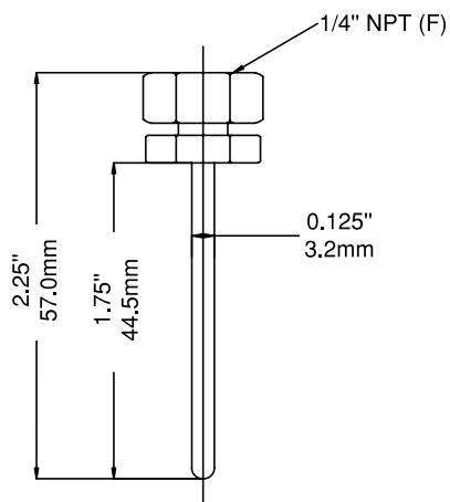
0.25" Test Plug
