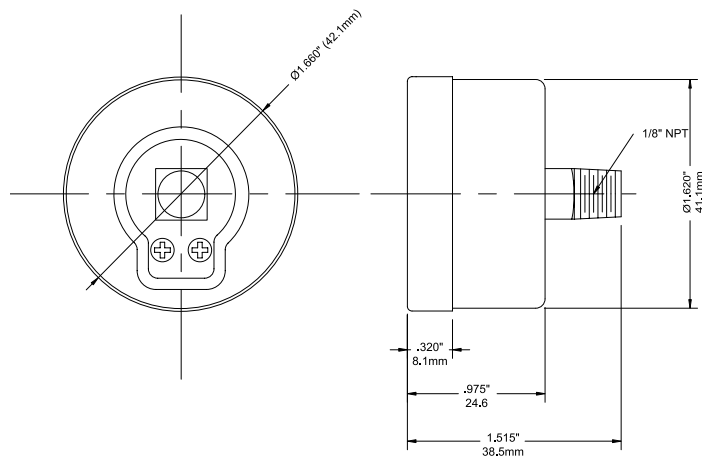
1.5" Back Connection
