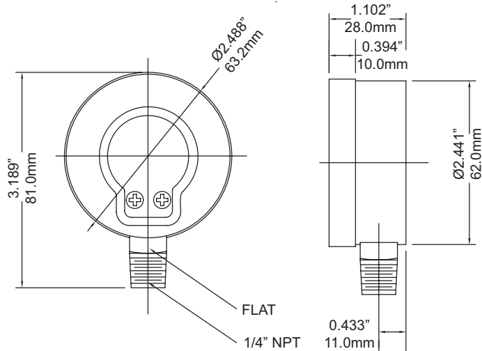
2.5" Bottom Connection
