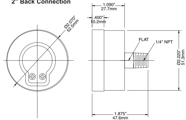
2" Back Connection
