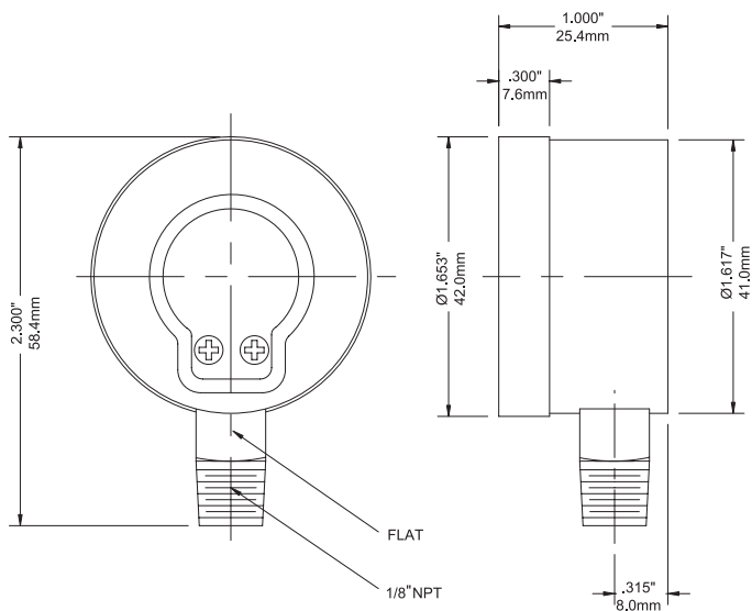
1.5" Bottom Connection
