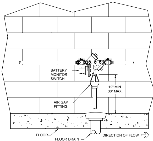
INDOOR INSTALLATION (Shown w/optional BMS)
