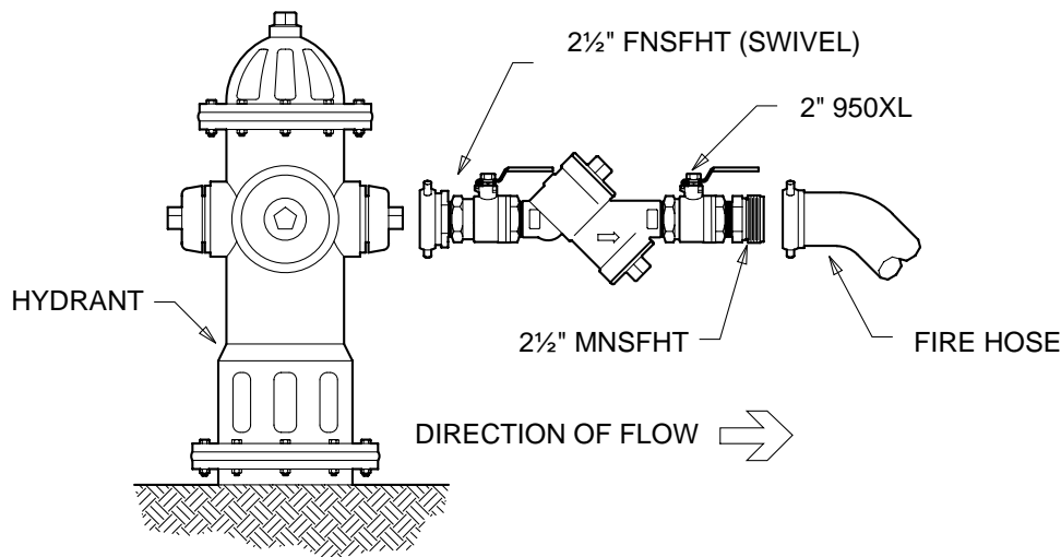
TYPICAL INSTALLATION
