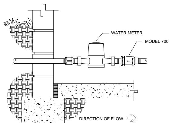
INDOOR INSTALLATION
