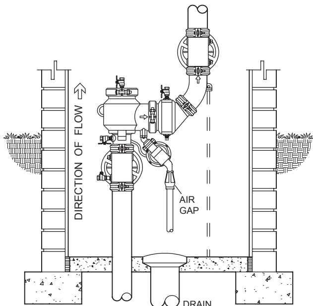
INDOOR INSTALLATION
