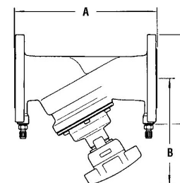
Flanged Model
