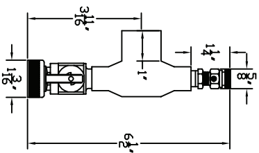
Vent/Purge Assembly: Supply
