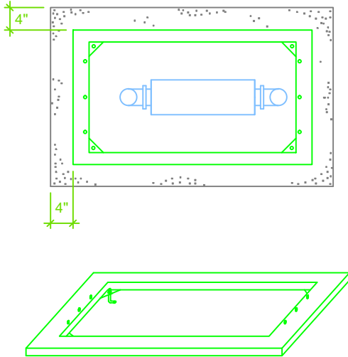
SMOOTH TOUCH ANCHOR BASE.
