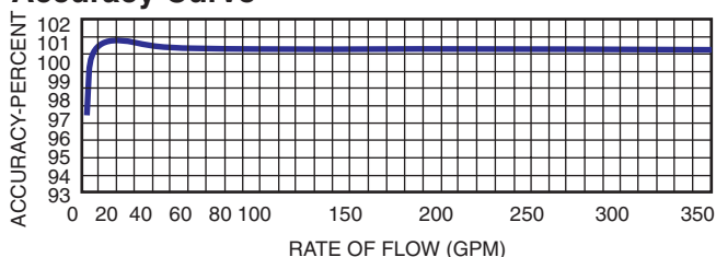
Accuracy Curve
