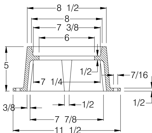
PAVING RING 4003
