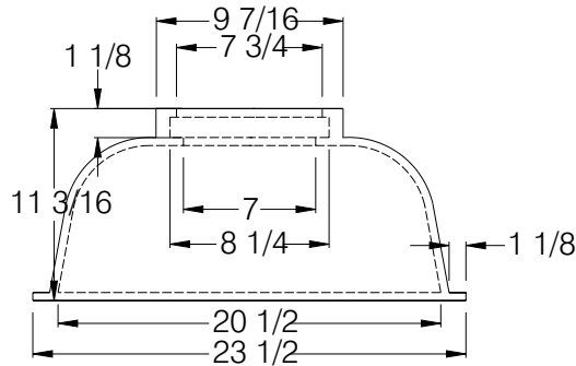
#160 BASE
