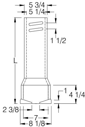
BOTTOM / EXTENSION
