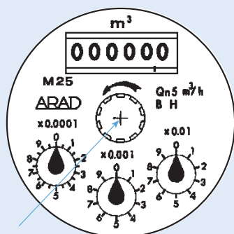
SERRATED WHEEL
