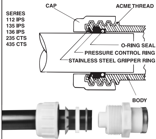
FIG.B FLO-LOCK COMPRESSION
