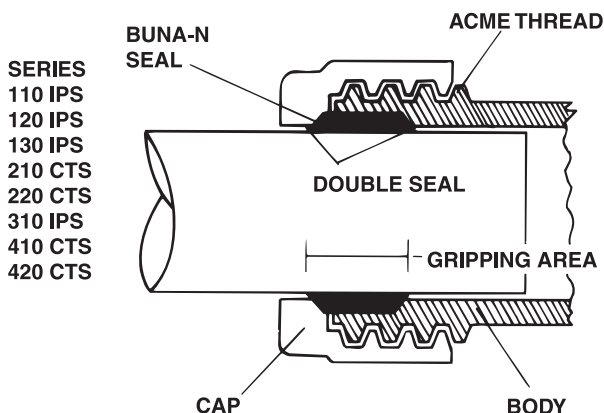
FIG.A STANDARD COMPRESSION
