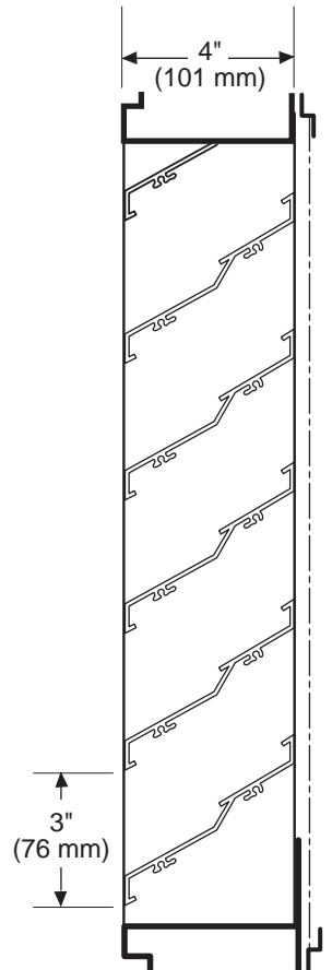
Channel Frame
