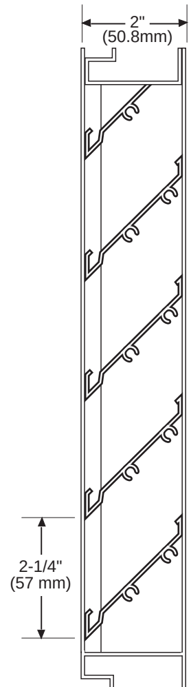
Channel Frame
