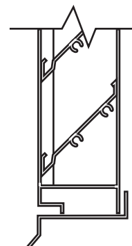
Sill Extension
