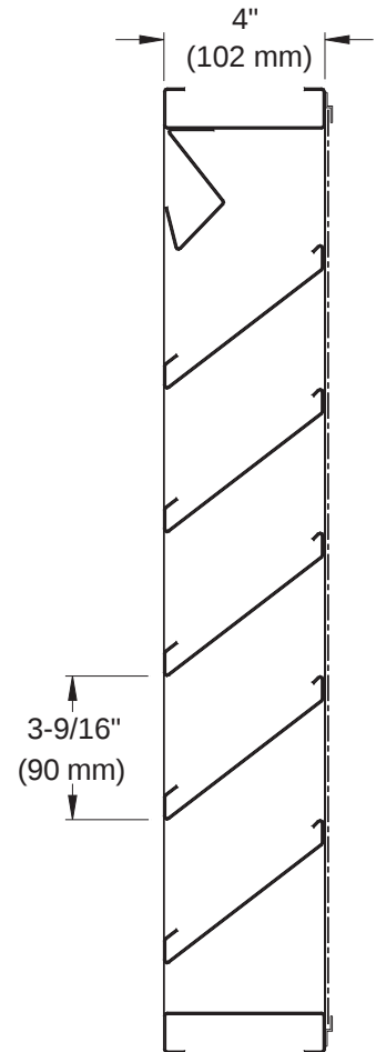
Channel Frame
