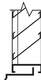
Sill Extension
