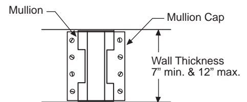
Detail F-F
