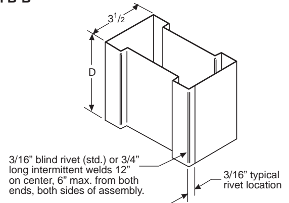
Assembled View
