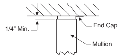
Detail G-G
