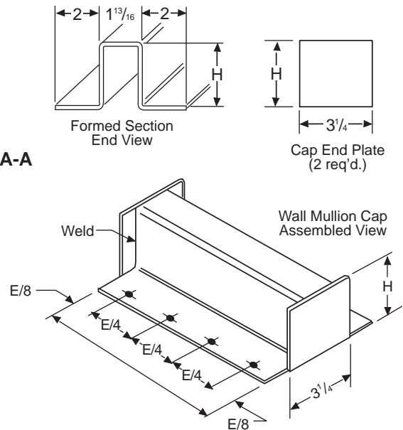
Formed Section View (2 req'd.)
