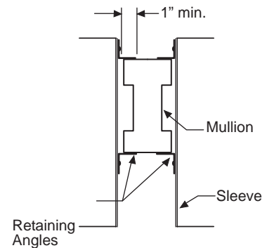
Detail E-E
