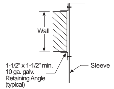
Detail D-D
