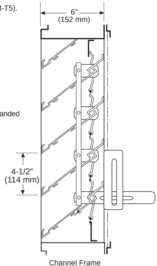
Channel Frame
