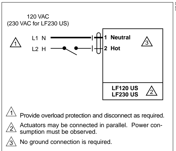
On-off wiring for LF120 US / LF230 US
