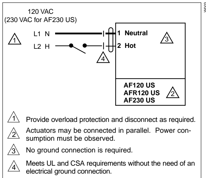
On-off wiring for AF120 US/AF230 US
