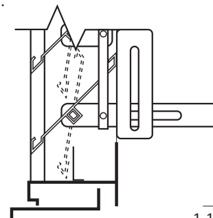
SILL EXTENSION
