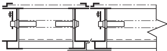
VISIBLE MULLION
