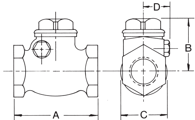
DIMENSIONS-INCHES
