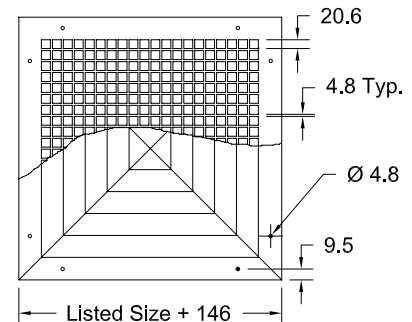
Face View (SG5500S-1 Model)
