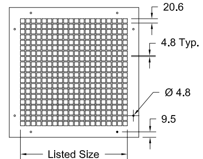
Face View (SG5LFP)
