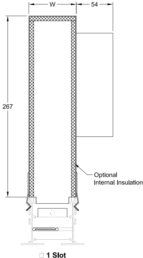
Plenum (Installed) End View
