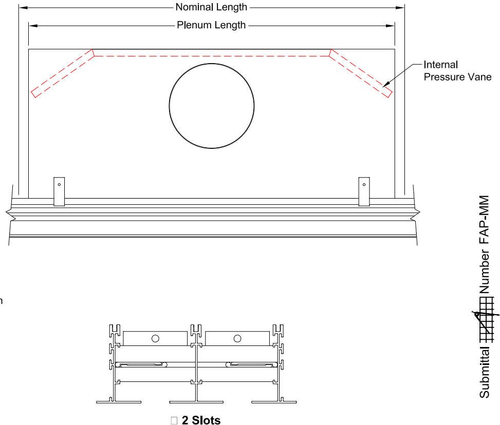
Plenum Side View
