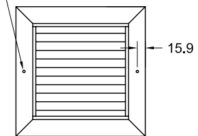
Face View ( Model DGSF ) Mounting Holes
