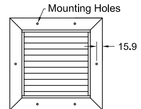
Face View ( Models: DGDF & DGLP )
