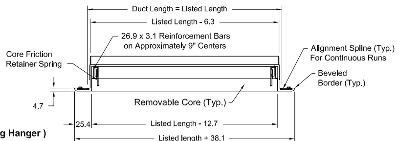
Side View
