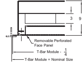
Cross Section: Diffuser Face
