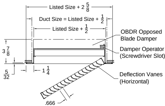
Option: SRHFD-1 FS ( Register - Filter Size - Surface Mount )
