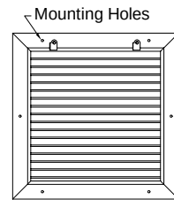
Face view (SRHF-1-GS & SRHF-1-FS)
