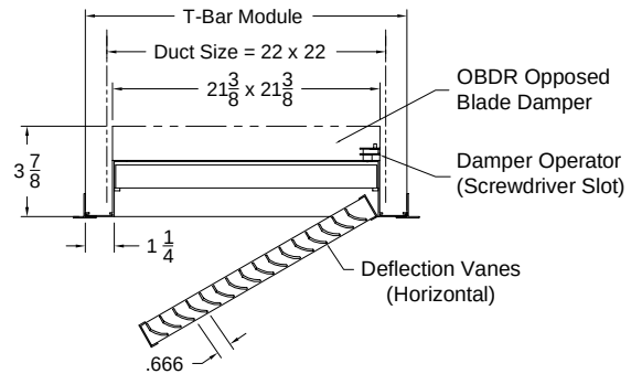
Option: SRHFD-6 FS ( Register - Filter Size - Lay in T-Bar )
