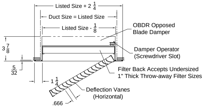
Option: SRHFD-1 GS ( Register - Grille Size - Surface Mount )
