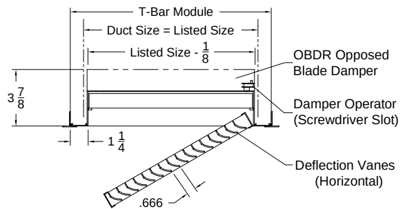
Option: SRHFD-6 GS ( Register - Grille Size - Lay in T-Bar )
