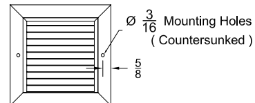
Face View (SRH-1 Model)
