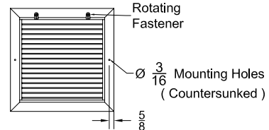
Face View (SRH-H-1 Model)
