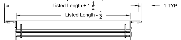
Side View (Both Models)
