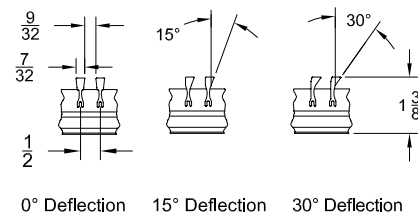
Air Pattern Deflectors
