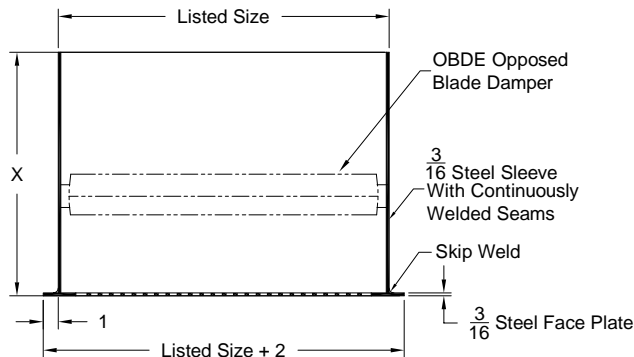
Model: SGRPD (Security Register - With OBDE Damper) (With Perforated Face)
