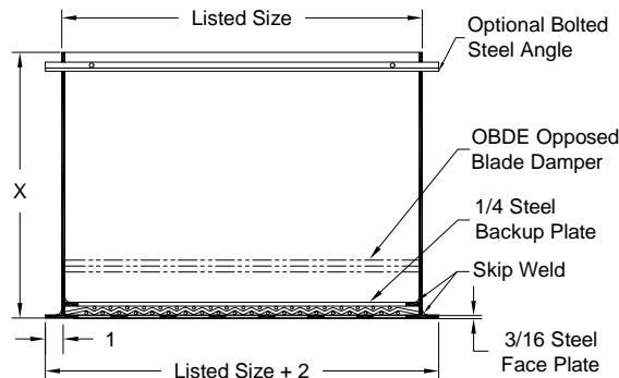
Model: SGSPD (Security Register - With OBDE Damper) (Square Holes - Mesh Screen Face)
