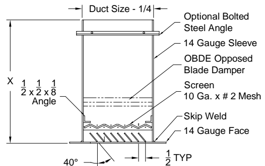
Model: SGRHD (Security Register - With OBDE Damper) (Fixed Louver Face)
