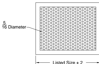
Model: SGRH (Security Grille - Fixed Louver Face)
