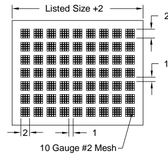
Face View (SGRP Model)
