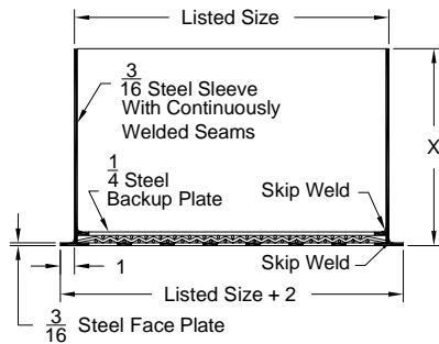
Model: SGRP (Security Grille with Perforated Face)
