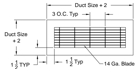
Face View (SGRH Model)
