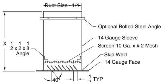
Model: SGRH (Security Grille - Fixed Louver Face)
