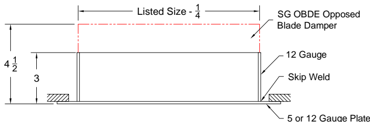
Model: SGLFPD (Minimum Security Register - With SG OBDE Damper - Lattice Face)
