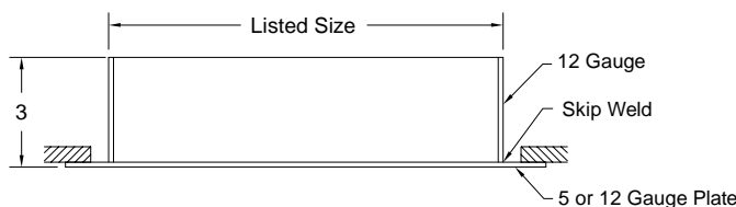
Model: SGLFP (Minimum Security Grille - Lattice Face Plate)
