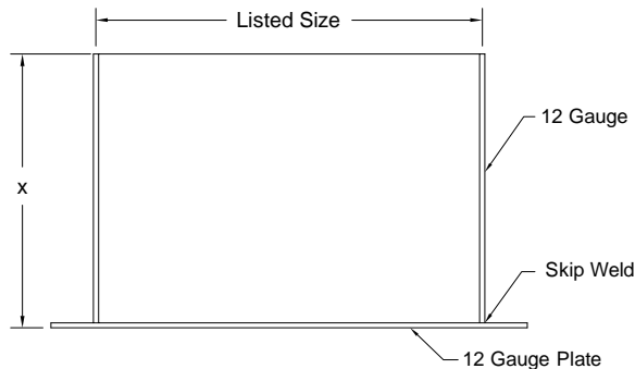
Model: SGLF (Medium Security Grille - Lattice Face)
