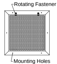
Face view ( RPF-1 GS & RPF-1 FS )
