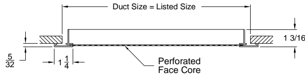
Model: RP-1 ( Perforated Grille - Surface Mount )
