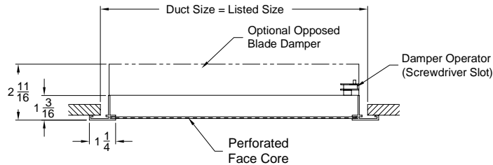
Model: RPD-1 ( Perforated Face Register - Surface Mount )
