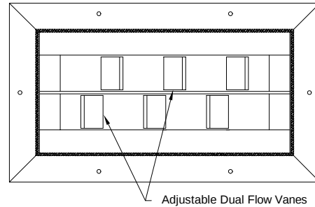
Model: RL-DF ( Roto Louver - Dual Flow Blades)
