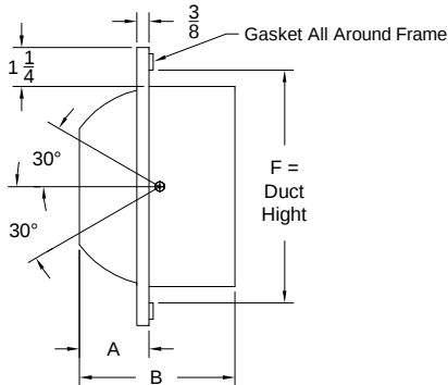
Shown Model: RL (Roto Louver - Standard Blades)
