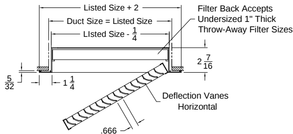
Model: RHF-1 FS ( Filter Return Grille - Filter Size - Surface Mount )
