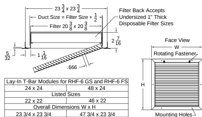
Model: RHF-6 FS ( Filter Return Grille - Filter Size - Lay in T-Bar )
