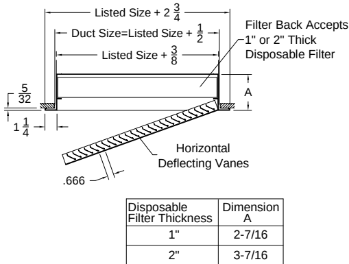
Model: RHF-1 FS ( Filter Return Grille - Filter Size - Surface Mount )
