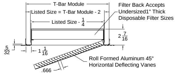
Model: RHF-6 GS ( Filter Return Grille - Grille Size - Lay in T-Bar )
