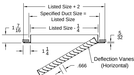
Model: RHED-1 ( Return Register - Surface Mount ) ( With OBDE Opposed Blade Damper )
