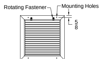
Face View ( Model RHE-H-1 )
