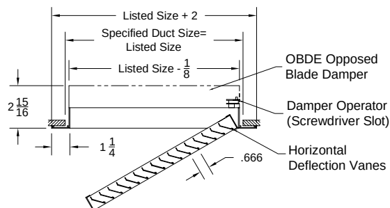
Model: RHE-HD-1 ( Return Register - Hinged Core ) ( With OBDE Opposed Blade Damper )
