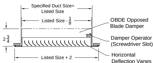
Model: RHED-1 ( Return Register - Surface Mount ) ( With OBDE Opposed Blade Damper )
