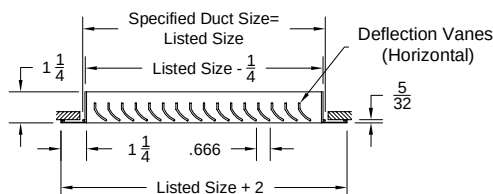
Model: RHE-H-1 ( Return Grille - Surface Mount - Hinged Core )
