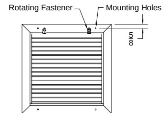
Face View (RH-H-1)
