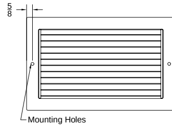
Face View ( RH-1 Model )
