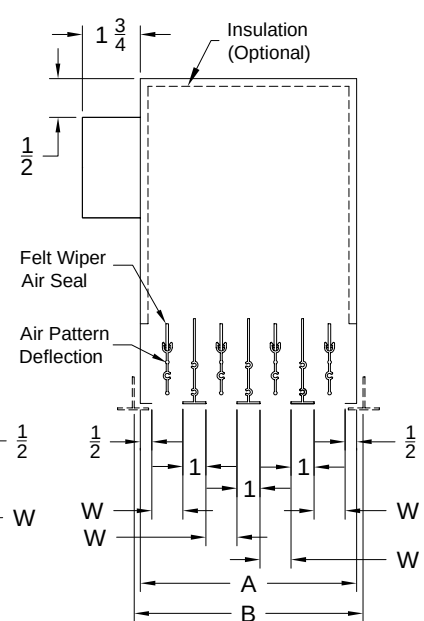
Model: PHPS(I)-6 4 Slots (-50, -75, -10, -15)
