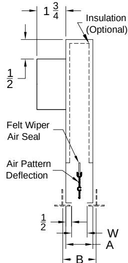
Model: PHPS(I)-6 1 Slot (-50, -75, -10, -15)
