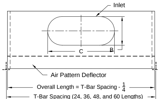
Front view (Models: PHCS & PHCR)
