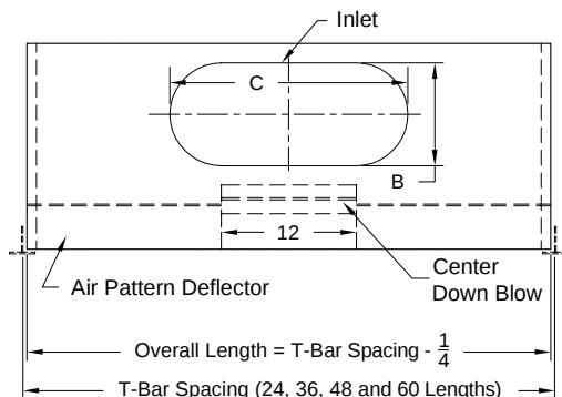
Front view (DB Models)
