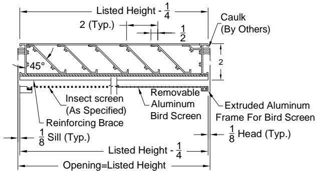
Model: OAL-2C (Type C - Channel Frame - 2" Depth)
