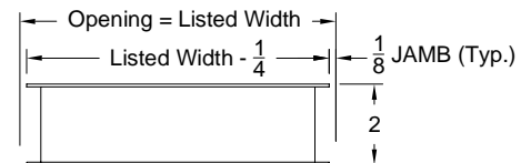
Model: OAL-2C (Side View)
