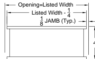
Model: OAL 4 C (Side View)
