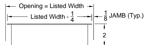
Model: OAL-2F (Side View)
