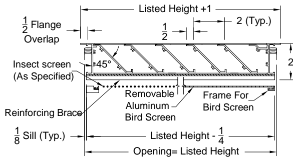
Model: OAL-2F (Type F - Flanged Frame - 2" Depth)
