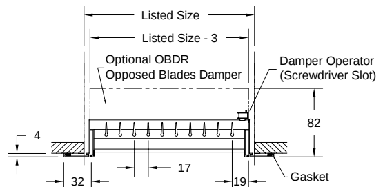
Option: V4004SDM-1 (Double Deflection Register) ( With OBDR Damper-Vertical Front Blades )
