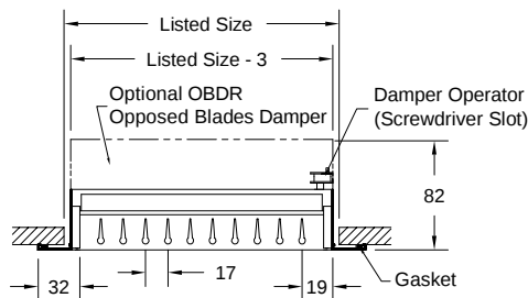
Option: H4004SDM-1 ( Double Deflection Register ) ( With OBDR Damper - Horizontal Front Blades )
