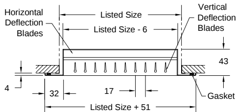
Option: H4004SDM-1 ( Double Deflection Register ) ( With OBDR Damper - Horizontal Front Blades )
