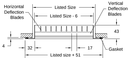
Model: V4004SM-1 ( Double Deflection Grille - Vertical Front Blades )
