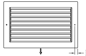
Face View ( LM-1 Model )
