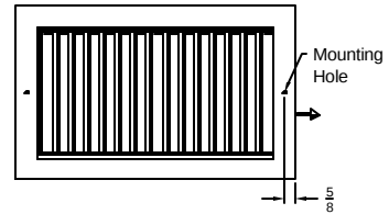
Face View ( S-1 Model )
