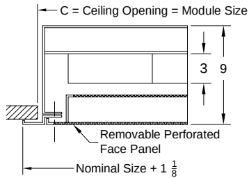
Model: HPL-PR-AL Border 1 ( Surface Mount )
