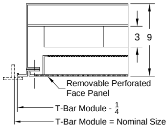
Model: HPL-PR-AL Border 6M (1 1/2 Inch Lay-In T-Bar)
