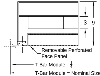
Model: HPL-PR-AL Border 6 (Standard Lay-In T-Bar)
