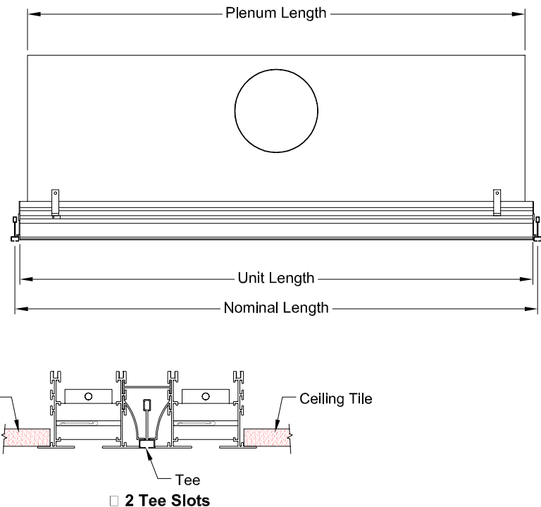
Plenum Side View
