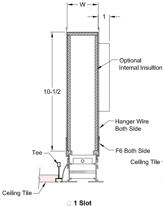
Plenum (Installed) End View
