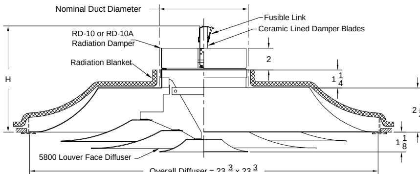
Model: 5800-6-FRS (Square Diffuser - Three Cones)
