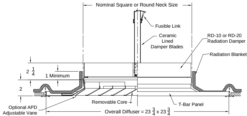
Model: 5500-6-FRS (Louver Face Diffuser - Square or Round Neck)
