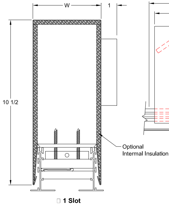
Plenum (Installed) End View
